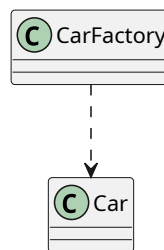
Figure 67: Example of dependency in UML class diagrams
